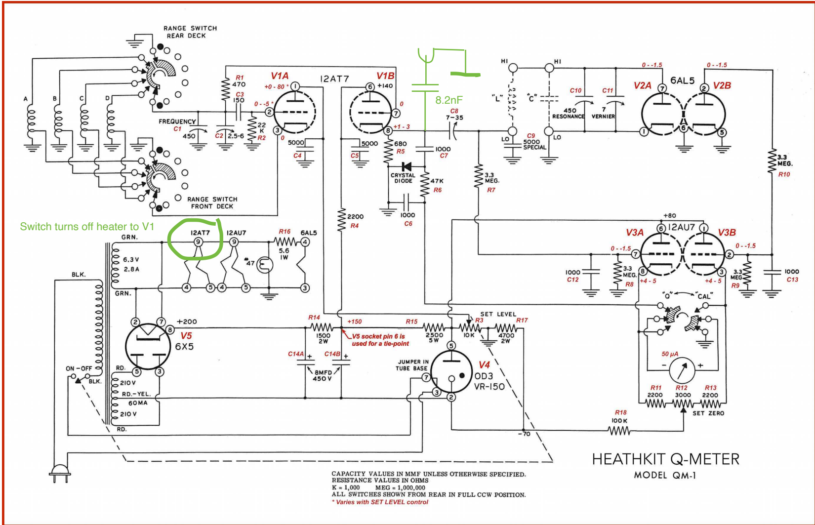
Figure 11: Heathkit QM-1 Schematic
